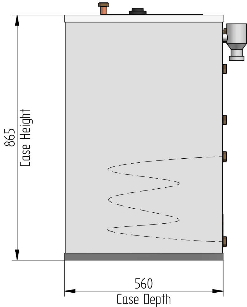
Inspection Lid (Cold Feed Cistern)
